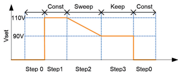
Sequence Waveform
