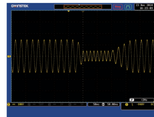
Voltage Fall
