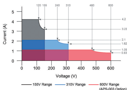
APS-7050 Output Operating Area
