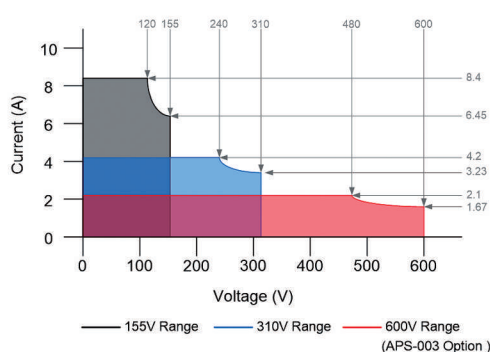
APS-7100 Output Operating Area
